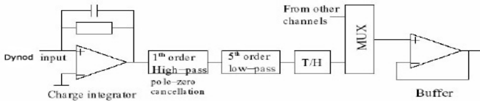
Figure 4. Single channel architecture [4].
