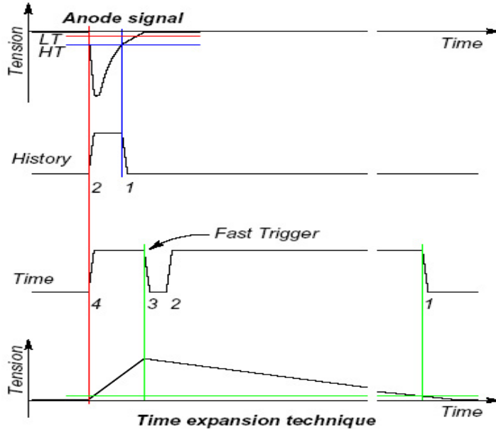
Figure 2. The time expansion technique [3].
