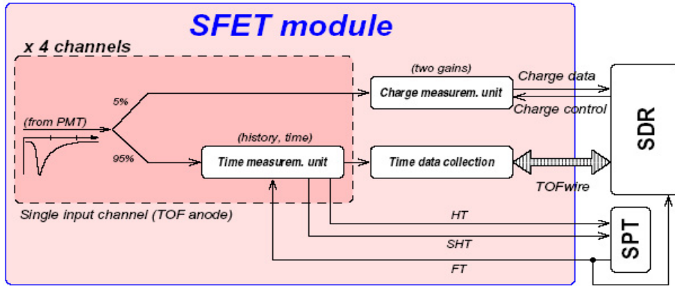
Figure 1. Anode signals received by the SFET module are split in two paths. The bigger fraction is used for the time measurement: the analog signal is compared to fixed thresholds [3].
