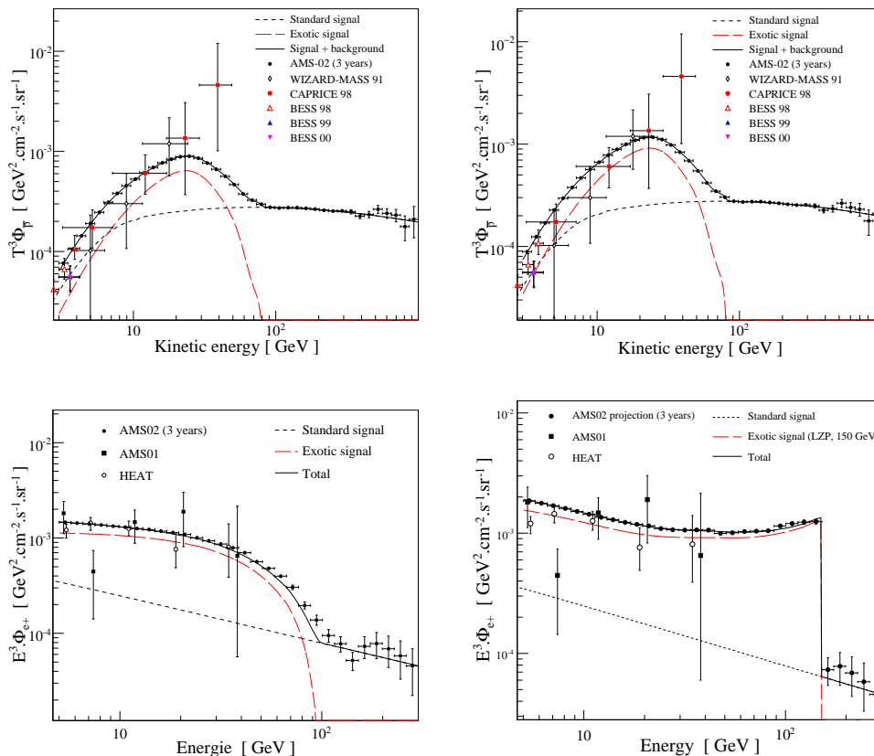
Fig. 1. Expected measurements of the e^+ flux for SUSY DM (a bino , left) and a LSP (right).
